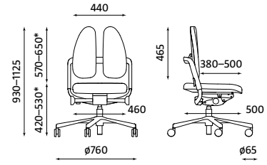
XENIUM OPERATIVE DUO-BACK IND-ST Weight | Waga 16.50 kg
