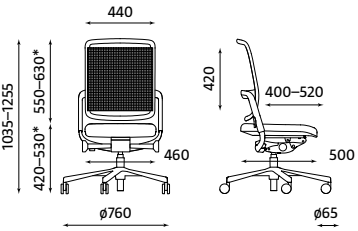
XENIUM OPERATIVE MESH IND-ST Weight | Waga 16.00 kg
