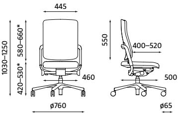
XENIUM OPERATIVE UPH IND-ST Weight | Waga 16.00 kg
