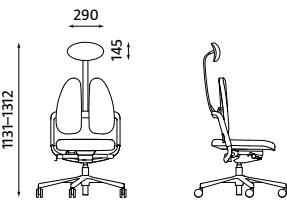
XENIUM OPERATIVE DUO-BACK ESP-ST HRUA Weight | Waga 16.90 kg
