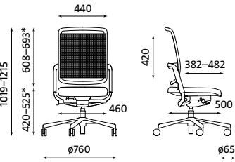
XENIUM OPERATIVE MESH ESP-ST Weight | Waga 13.90 kg
