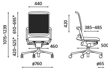
XENIUM OPERATIVE MESH DNP-ST Weight | Waga 15.90 kg
